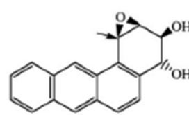
3S,4R,1R,2S-BaA-diol epoxide
