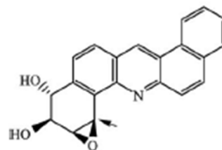
10S,11R,8R,9S-DB[a,h]A-diol epoxide
