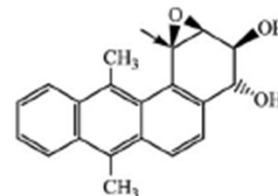
3S,4R,1R,2S-DMBA-diol epoxide
