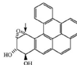
11R,12S,13S,14R-DB[a,l]P-diol epoxide
